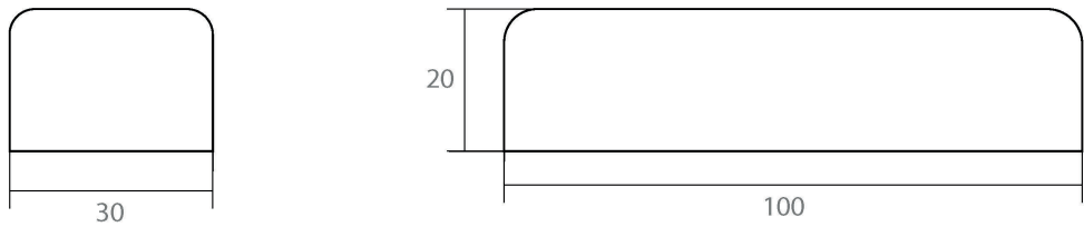
TRANSFORMER DIMENSIONS
