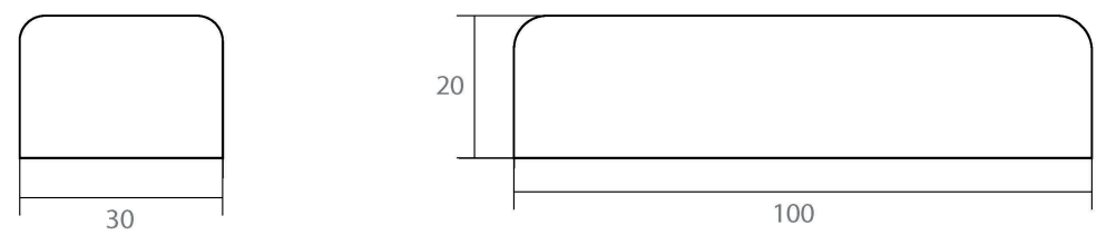
TRANSFORMER DIMENSIONS
